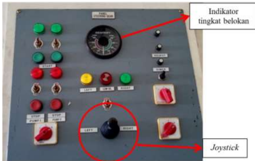
Gambar 4. Panel Steering Gear di Anjungan
